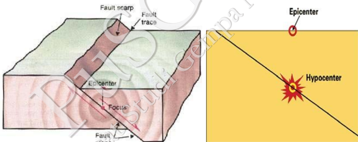
Gambar VI-5. Ilustrasi model sumber gempa sesar/ fault ( http://earthquake.usgs.gov/learn/glossary/ )
