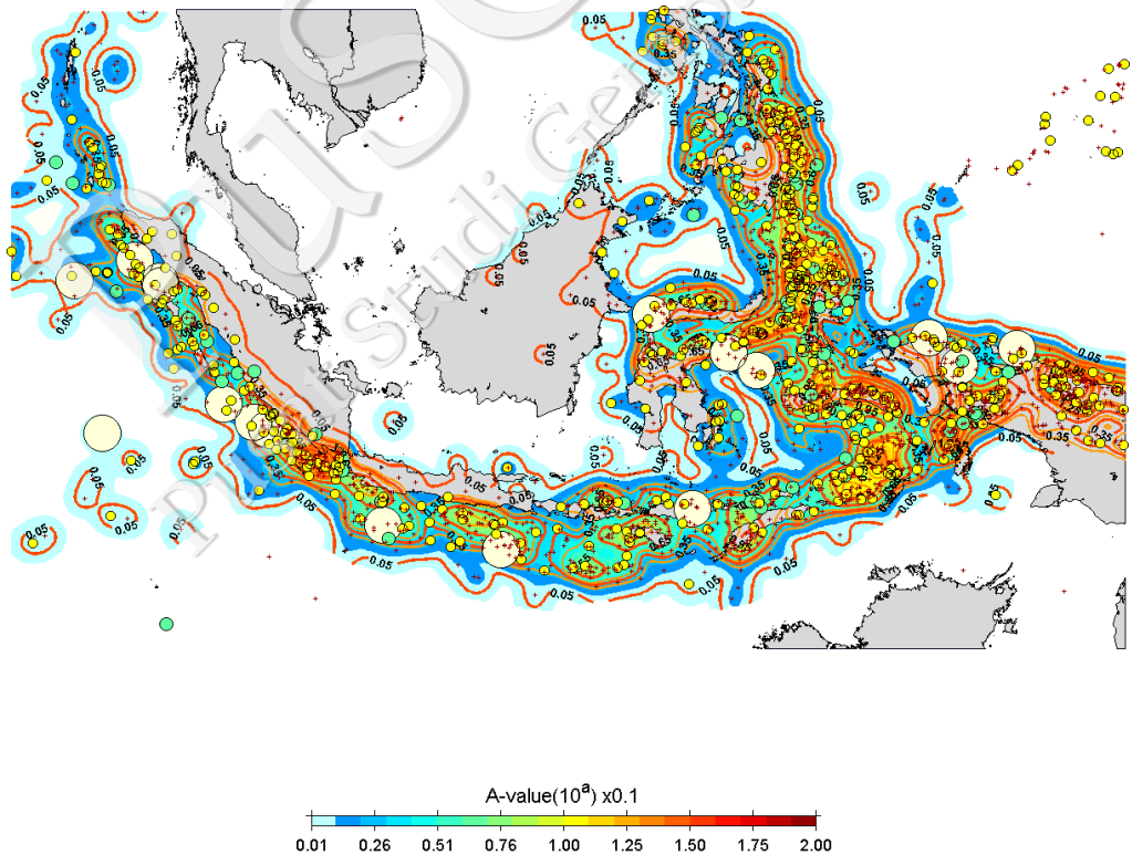
Map A-value (1991-2016; H:0-60km)
