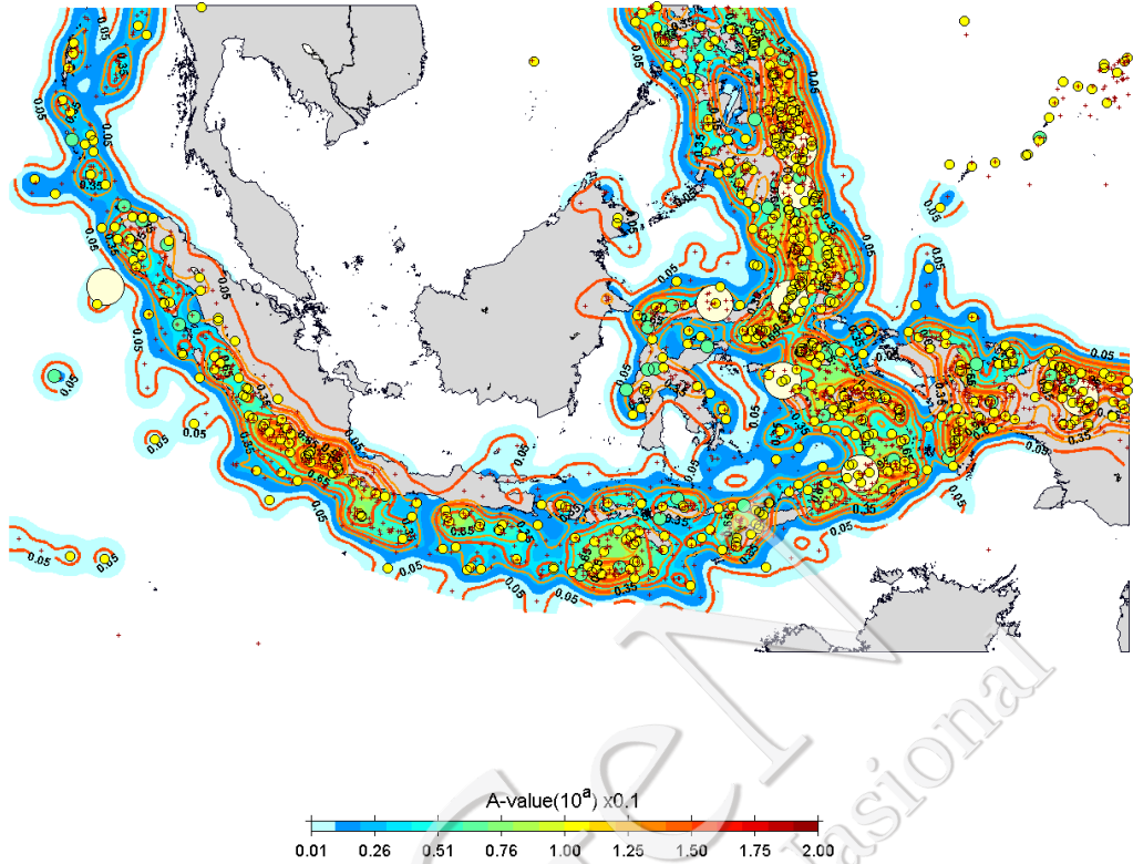
Map A-value (1963-1990; H:0-60km)
